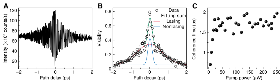
Fig. 3. Coherence time measurement. (A) Raw data of intensity as a function of path delay at pump power of 250 \mu\text{W} . (B) Visibility as a function of path delay at pump power of 250 \mu\text{W} . Two-peak Gaussian fitting is used to extract the contribution of lasing mode. (C) Coherence time as a function of pump power.
